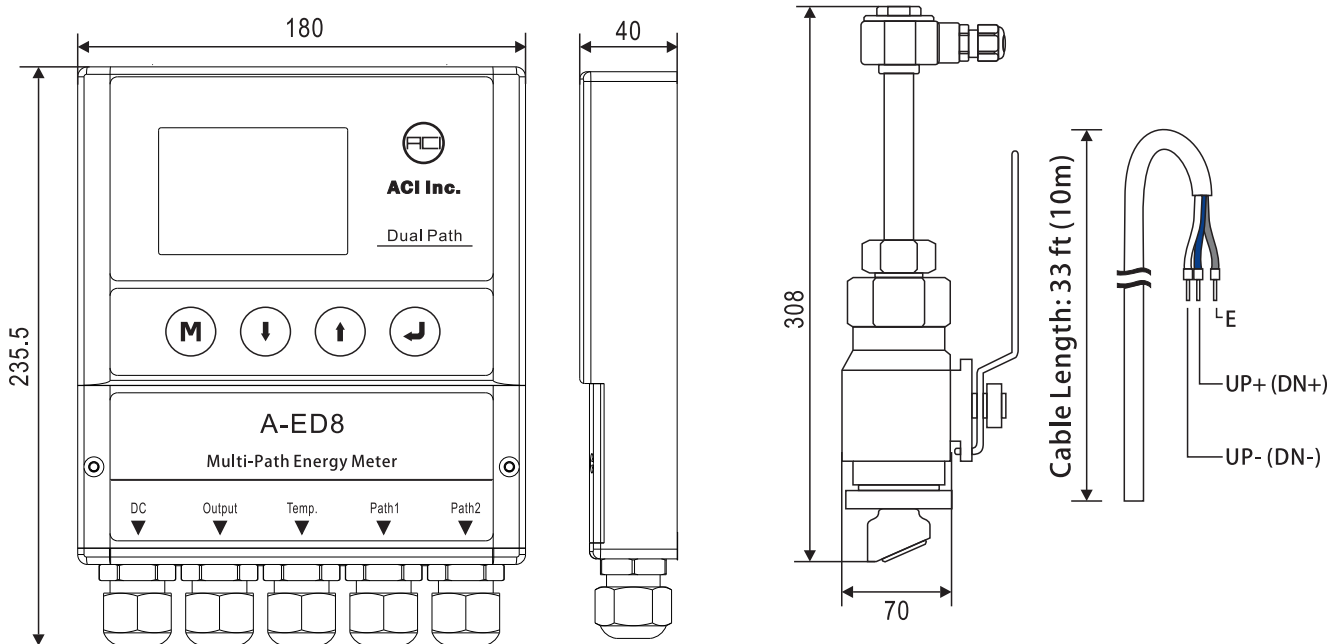
Transmitter dimensions(mm)
